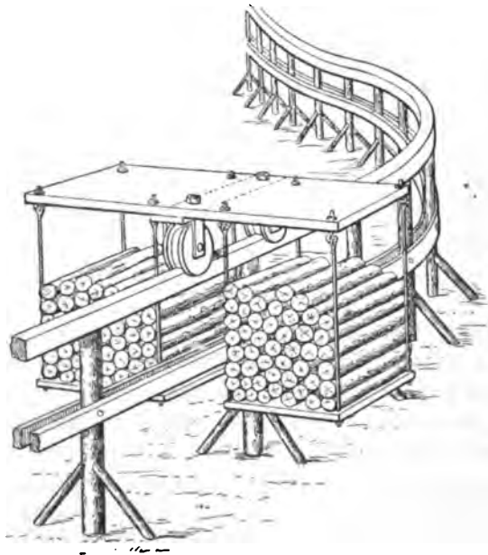
Fig. 284A.—De Coulon's monorail at Neufchateau. After Mathey. ( Cf. p. 334.)
